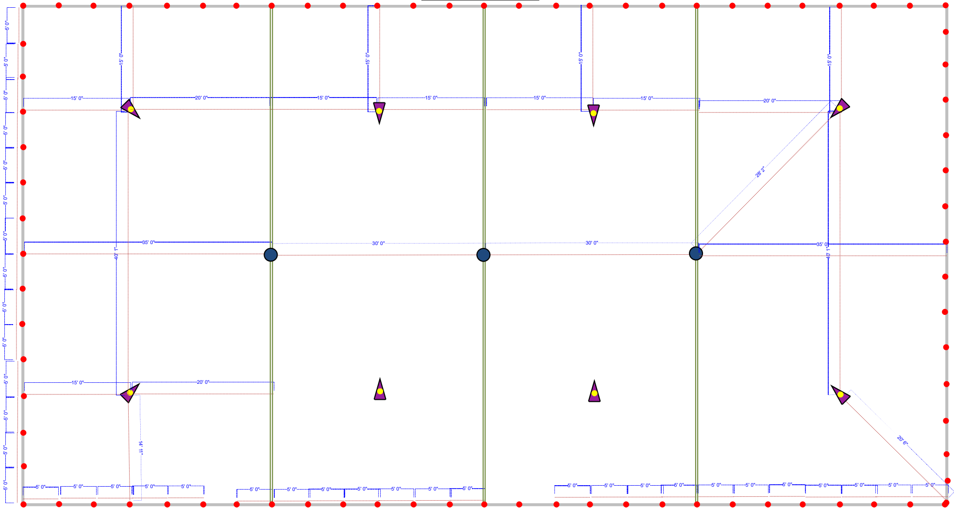
70' x 130' Pole Tent - Pole Placements
